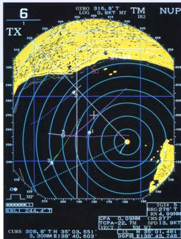
Overlay display of coastlines and other ship's tracks on radar display in ARPA/Plotter combined mode
